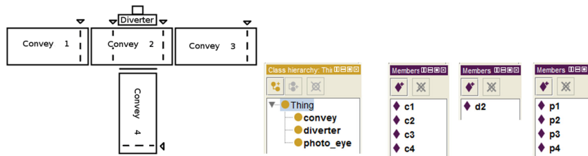
Fig. 3. A fragment of an airport baggage handling system (left) and its ontological representation (Right).
