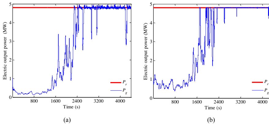
Fig. 11. Generated and reference power (MPC): a) without supervisor, b) with supervisor.
