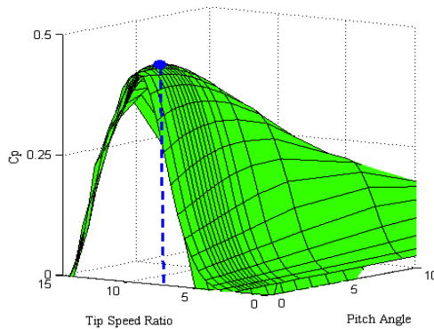
Fig. 3. Power coefficient curve.
