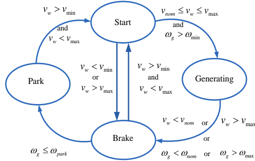
Fig. 5. Representation of the operational states and conditions.
