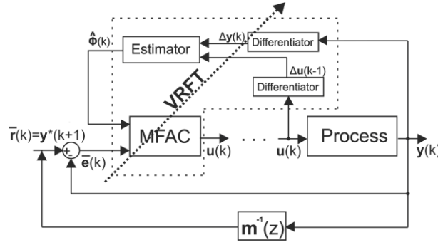
Fig. 1. Structure of mixed MFAC-VRFT CS
