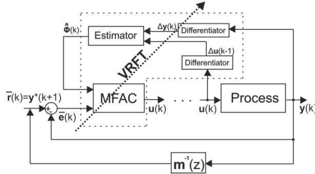
Fig. 1. Structure of mixed MFAC-VRFT CS
