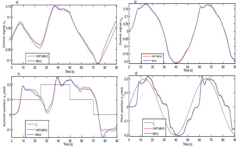
Fig. 2. Experimental results expressed as CS responses in the MIMO scenario: control signals u_1 and u_2 , process outputs y_1 and y_2 and references trajectories y_1^* and y_2^*
