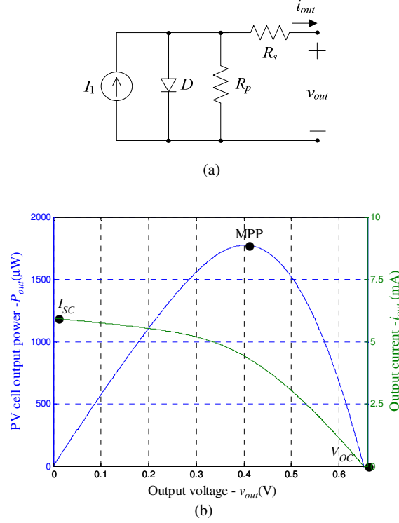
Fig. 1. PV cell: a) Equivalent electric circuit; b) Example of typical current and power curves.
