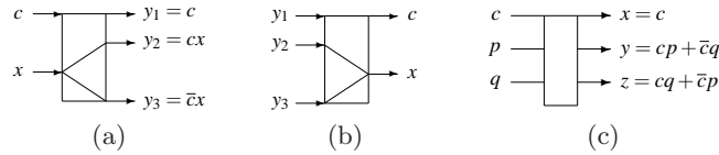
Fig. 24. (a) Switch gate. (b) Inverse switch gate, where c = y_1 and x = y_2 + y_3 under the assumption (y_2 \rightarrow y_1) \wedge (y_3 \rightarrow \bar{y}_1) . (c) Fredkin gate.
