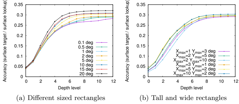
Fig. 3: Accuracy per lookup depth
