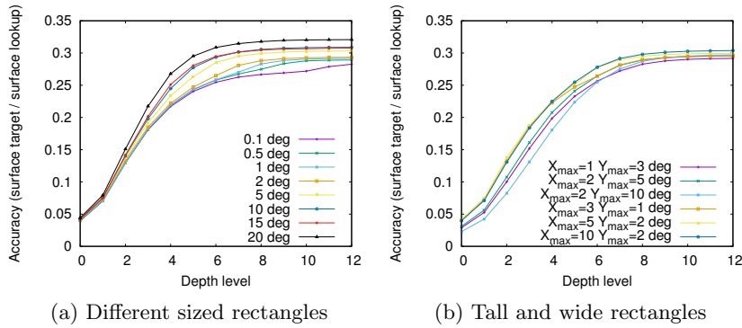
Fig. 3: Accuracy per lookup depth
