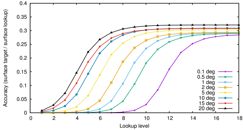
Fig. 2: Accuracy per level of different sized rectangles
