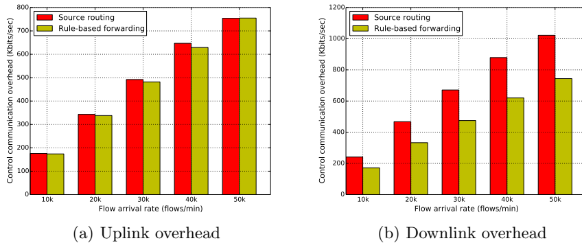
Fig. 7. Control overhead for a single switch.
