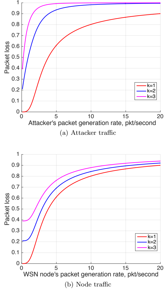
Fig. 5. Impact of packet generation rate on packet loss rate
