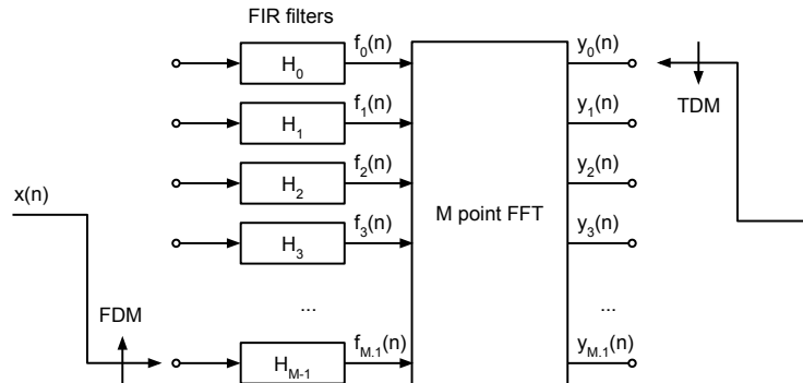
Fig. 3. PFB channelizer.
