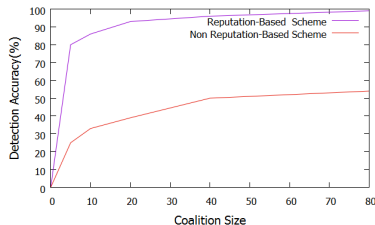
Fig. 2: Detection Accuracy
