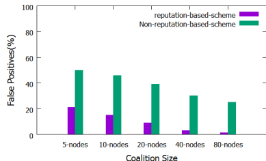
Fig. 4: False Positives
