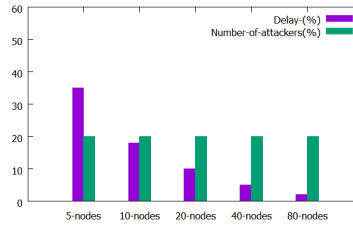
Fig. 3: Detection Delay
