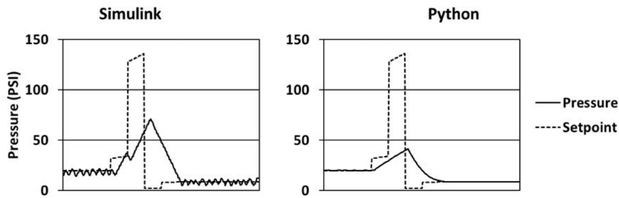
Figure 12. Python and Simulink simulations under attack.
