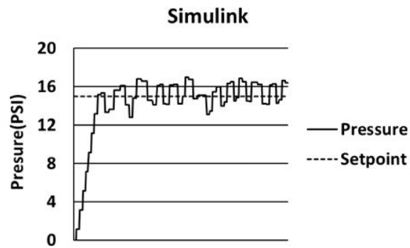
Figure 10. Simulink system (normal operation).
