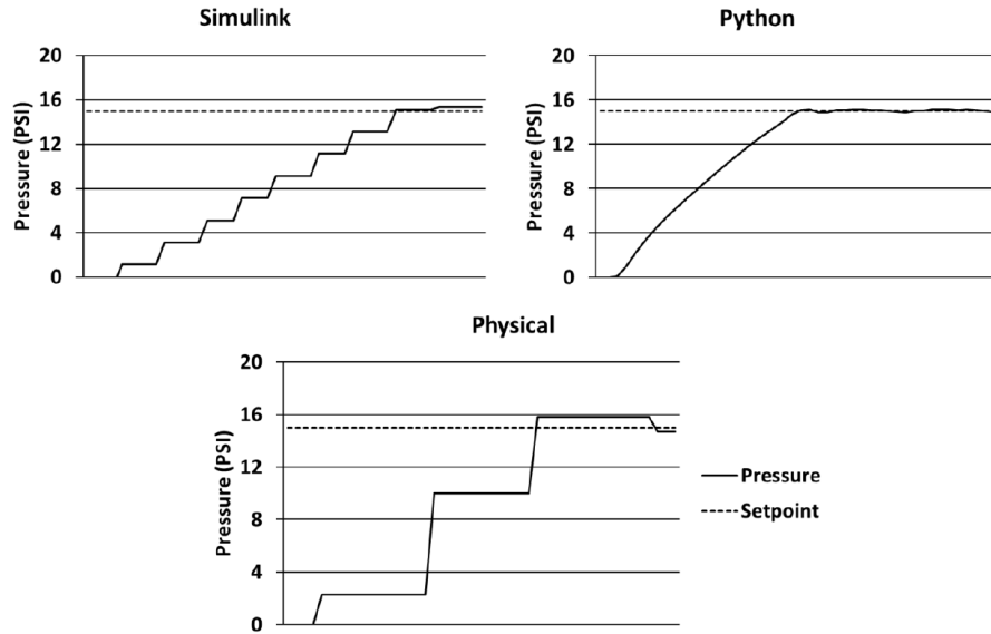
Figure 11. System startup.
