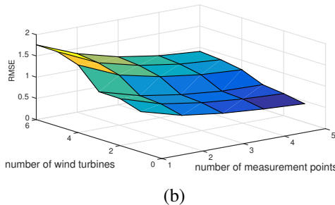
Fig. 1. RMSE of the emergence estimate as a function of (a) the standard deviations \sigma_x and \sigma_a of the model uncertainties and the standard deviation \sigma_{r,\bullet} of the source separation system on the first dataset and (b) the number of measurement locations and wind turbines on the second dataset. The central difference Kalman filter is used.
