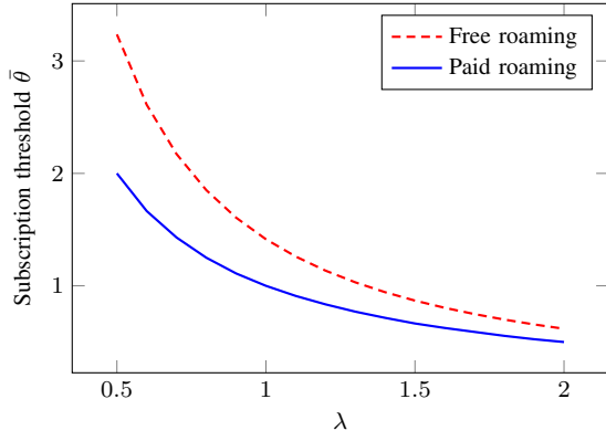
Figure 3. Subscription threshold \bar{\theta} , in terms of \lambda : users with \theta > \bar{\theta} subscribe to the service.
