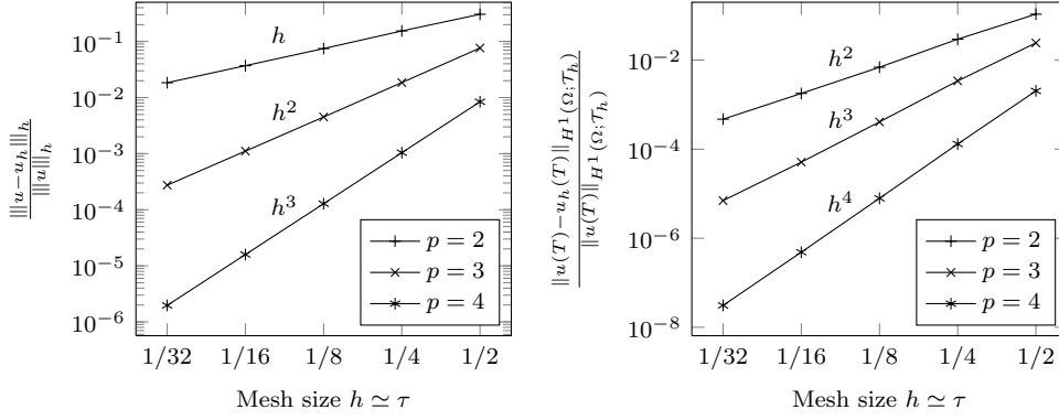
Fig. 1 Relative errors in approximating the solution of the problem of section 8.1 using uniform meshes and time partitions with \tau \simeq h and p = q + 1 . It is seen that the optimal convergence rates \| \|u - u_h\| \|_h \simeq h^{p-1} + \tau^q are achieved. The final time error, as measured in the broken H^1 -norm, also converges with the optimal rate \|u(T) - u_h(T)\|_{H^1(\Omega; \mathcal{T}_h)} \simeq h^p .
