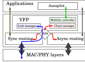
Fig. 3. Representation of the cross-layer framework.
