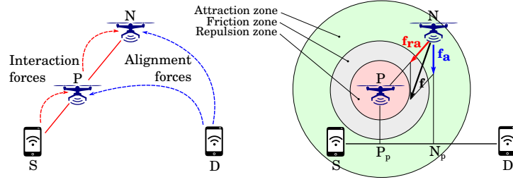
Fig. 2. (left) Principles of virtual forces applied on nodes P and N in a communication chain, (right) detailed forces on N (note that friction f_{fr} is non-existent in this case).
