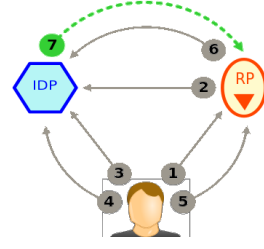
Figure 1: UnlimitID Information Flow
