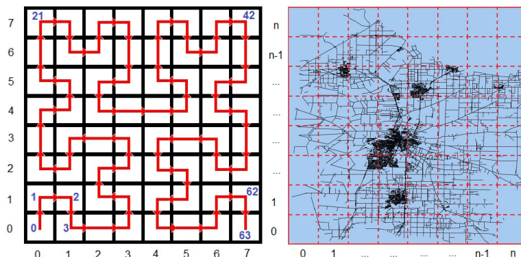
Figure 5: Hilbert indexing of spatial units
