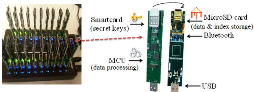
Figure 7: Secure tokens
