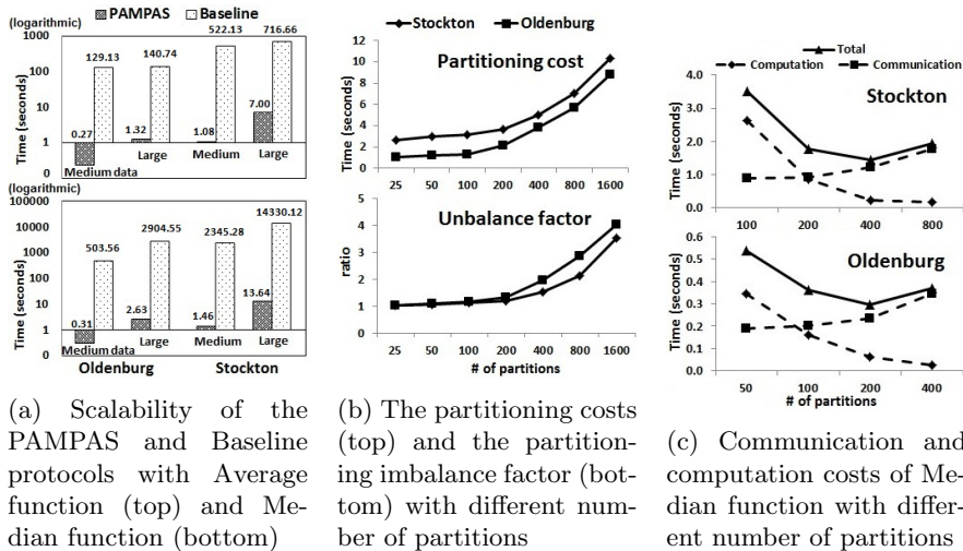
Figure 9: Performance evaluations
