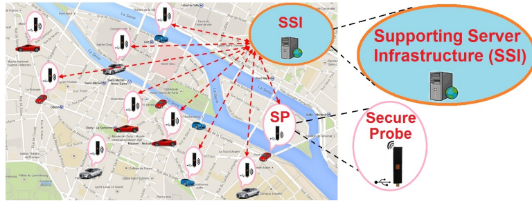
Figure 1: System architecture
