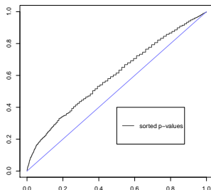
FIGURE 14. Sorted p-values p_{KS} DTM-KS.
