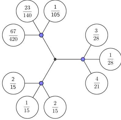
FIGURE 1. \mu
