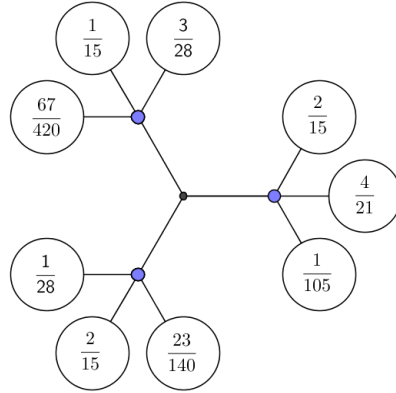
FIGURE 2. \nu
