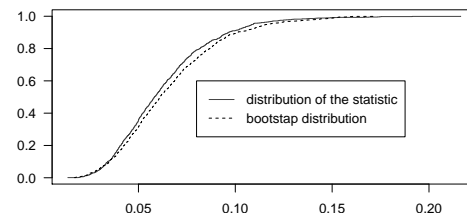
■ Figure 3 DTM-signature estimates, m = 0.05 ■ Figure 4 Bootstrap validity, v = 10 , m = 0.05
