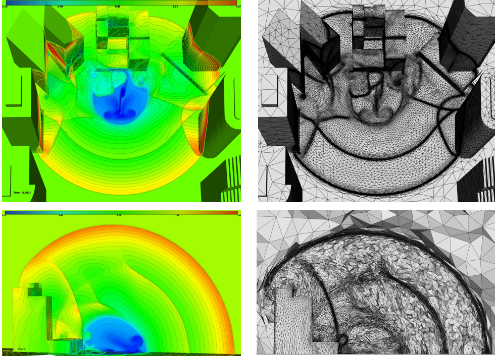
Figure 17: City blast . Density solution (left) at a -dimensioned time T = 15 and final adapted mesh (right) containing 487,440 vertices and 2,802,472 tetrahedra obtained with the \mathbb{P}_1 -conservative interpolation for n_{\text{adap}} = 128 .
