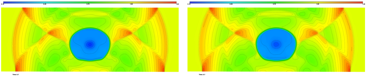
Figure 13: Spherical blast. Density solution at a-dimensioned time T = 0.7 obtained with the \mathbb{P}_1 -conservative interpolation (left) and the \mathbb{P}_1 interpolation (right) for n_{\text{adap}} = 16 and N_{\text{ver}} = 240K .
