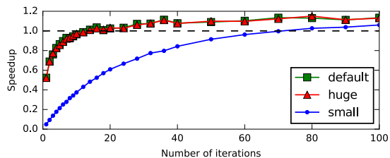
Figure 11: Speedup of page migration (synthetic benchmark)
