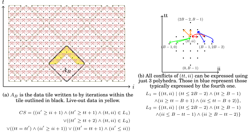
Fig. 7. Fig.7(a) shows diamond tiling for a stencil with flow dependences (1, -1) , (1, 0) and (1, 1) . If B is the tile size, the live-out set is a union of polyhedra L_1 and L_2 . The last two disjuncts in the conflict set CS represent conflicts due to flow dependences. The first two specify additional conflicts due to live-out values.
