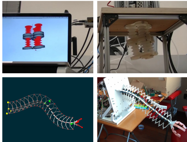
Fig. 5. Top: Control from inverse simulation of two Fetch platforms stacked for the Soft Robotic Toolkit 2015 competition. Bottom: Simulation of Flexo (left) and the real robot (right).
