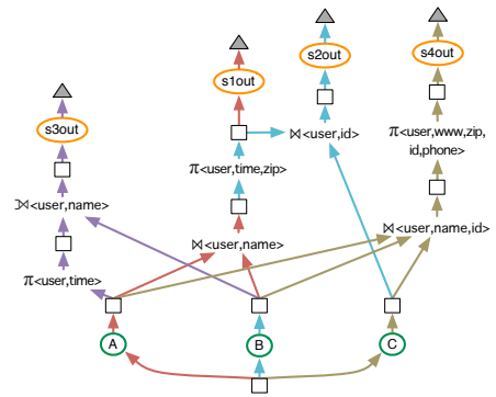
Figure 3: Possible REG for the EG in Figure 2.
