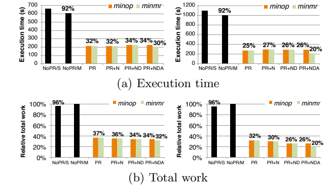
Figure 6: PigReuse evaluation using workload W_1 (left) and W_2 (right).
