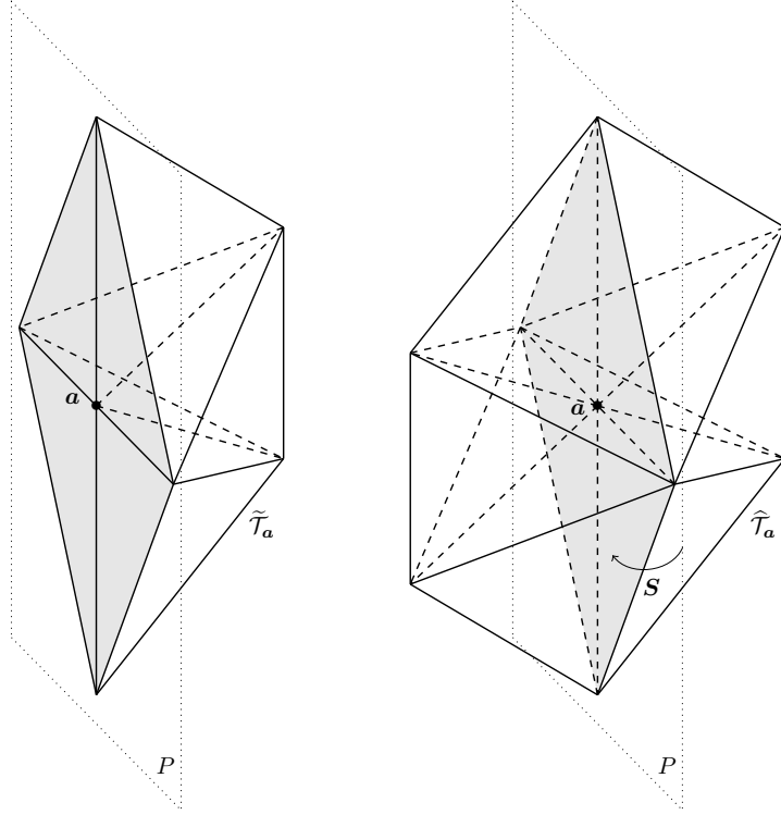
Figure 3: Left: boundary patch \mathcal{T}_a of the left panel of Figure 2 mapped by \mathbf{T} to the flattened patch \tilde{\mathcal{T}}_a lying in the half-space of \mathbb{R}^3 determined by the plane P ; right: patch \tilde{\mathcal{T}}_a mapped by the symmetry \mathbf{S} over the plane P and the resulting interior patch \hat{\mathcal{T}}_a
