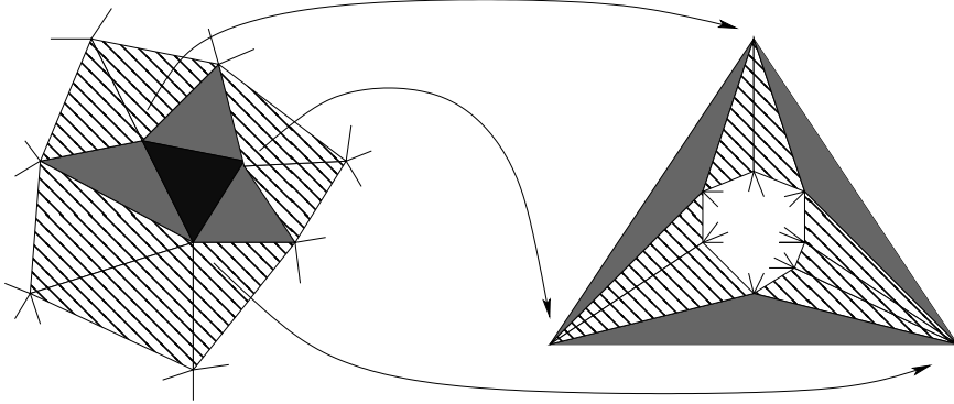
Figure 5: Left: original patch \mathcal{T}_\mathbf{a} \cap \partial\omega_\mathbf{a} locally around K_* \cap \partial\omega_\mathbf{a} (highlighted in dark grey), the three triangles K' \cap \partial\omega_\mathbf{a} for which the tetrahedron K' shares an interior face with K are highlighted in light grey, and the triangles K' \cap \partial\omega_\mathbf{a} for which the tetrahedron K' shares only an interior edge with K are dashed; Right: mapping by the homeomorphism to a triangulation of the unit triangle T in \mathbb{R}^2 ; the polygon at the heart of T is the image by the homeomorphism of all the triangles K' \cap \partial\omega_\mathbf{a} where K' only shares the vertex \mathbf{a} with K_* .
