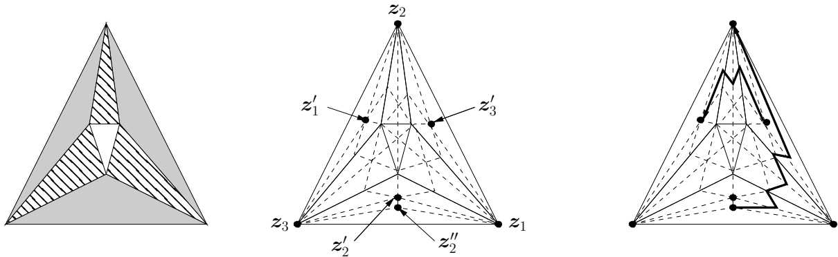
Figure 6: Left: original triangulation in the simple case where there is only one dashed triangle at each of the three vertices \{z_1, z_2, z_3\} ; Center: refined triangulation at the end of Step (2) showing the barycenters \{z'_1, z'_2, z'_3\} and the newly created one z''_2 ; Right: final refined triangulation where now all the vertices have even degree.
