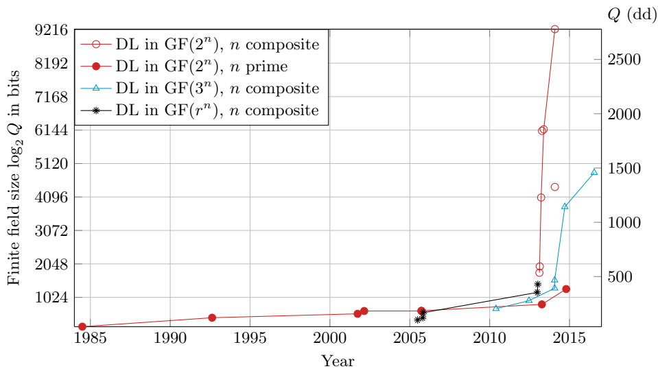
FIGURE 9.4 Records of DL computation in fields \mathbb{F}_{2^n}, \mathbb{F}_{3^n}, \mathbb{F}_{r^n} of small characteristic, with n prime or composite. All the fields \mathbb{F}_{2^n}, \mathbb{F}_{3^n} with n composite are target fields of supersingular pairing-friendly (hyper-)elliptic curves.
