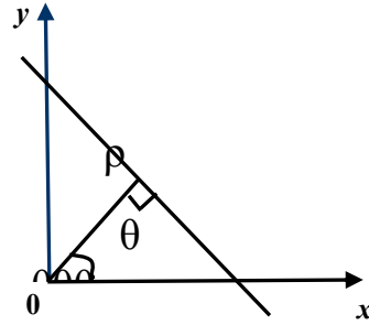
Fig.3. Point (x, y) was transformed to \theta - \rho parameter space
