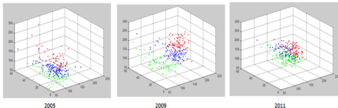
Fig3. Clustering results
