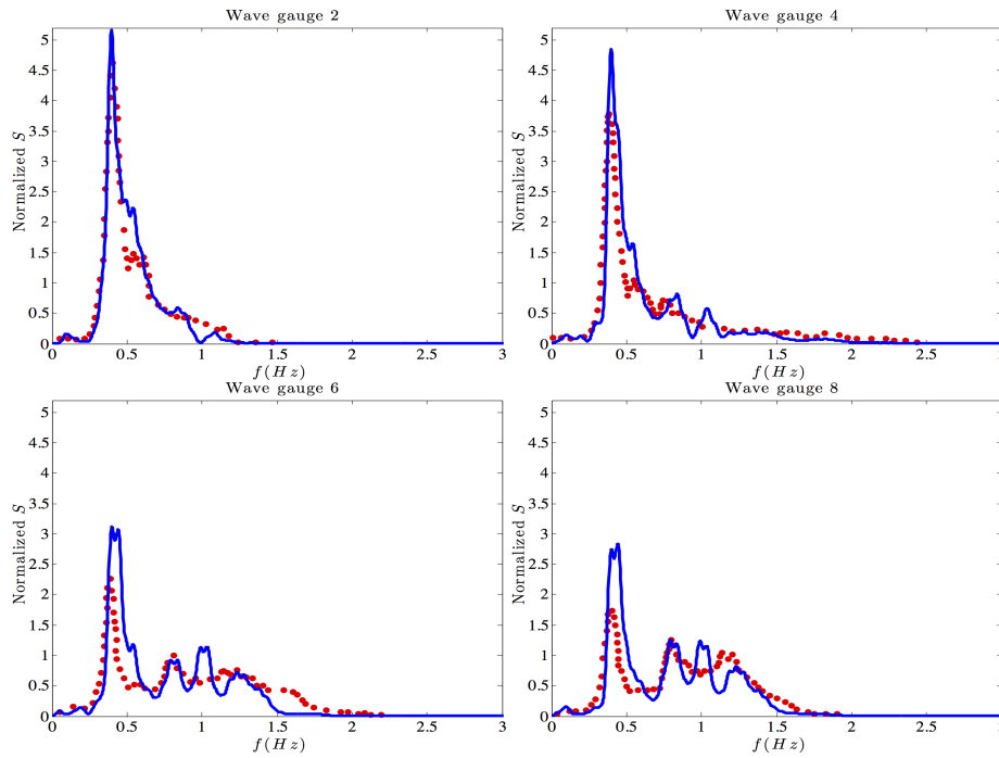
Figure 10: Power spectrum of the surface elevation for the wave gauges 2,4,6 and 8.
