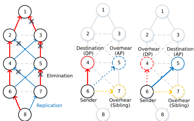
(a) Packet Replication procedure.
