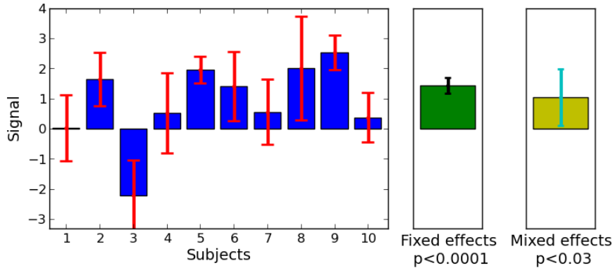
Figure 3: Illustration of the difference between fixed- and mixed-effects inference: Given n = 10 observations associated with a given level of uncertainty (left), one can perform a fixed-effects inference that ignores cross-subject variability of the observations and thus leads to population effects with tight uncertainty (middle), or consider this variance and then obtain wider uncertainty estimates (right). Only the mixed effects model yields a valid inference on the population from which the observations were sampled.
