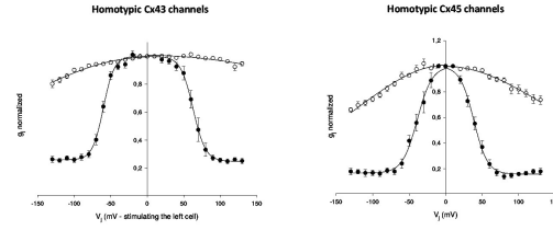
Figure 1: Dependence of the normalised gap junction conductance g_{j,\infty} (lower curves) and g_{j,inst} (upper curves) on junctional potential V_j for homotypic Cx43 and Cx45 channels.
