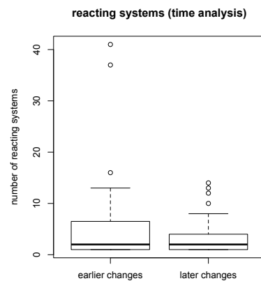
Fig. 4 Box plots for the reacting systems separated by earlier and later API changes.
