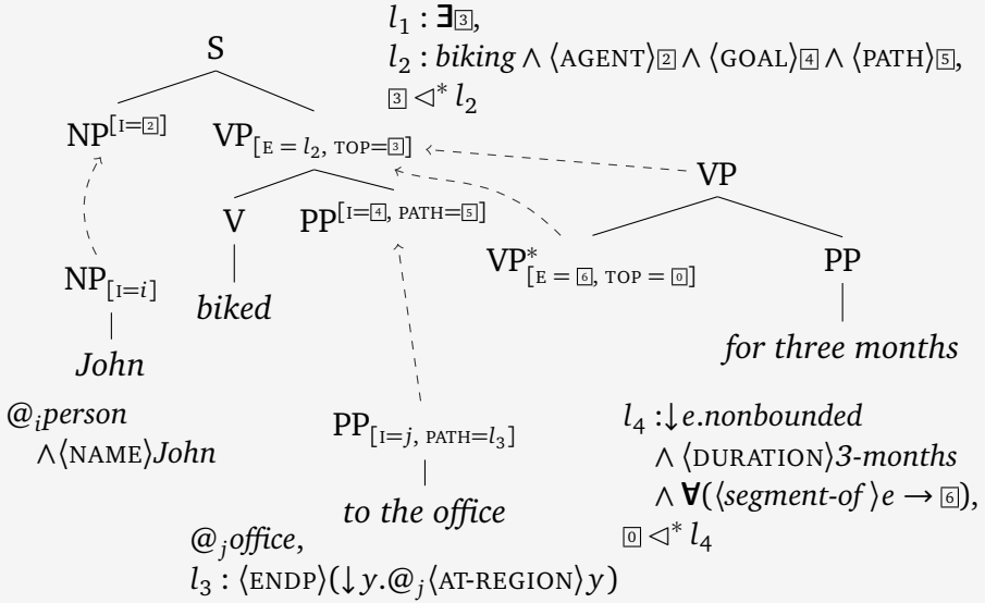
Figure 8 Derivation for (24)
