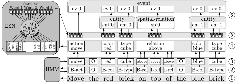
Fig. 2: Processing of a simple example sentence. First, IOB2 tags ② are generated (e.g. move \rightarrow B-action ) from the input sequence ①. Then the HMM creates chunk labels ③ for words ① (e.g. on \rightarrow above ). Afterwards the identified chunks ② are merged (e.g. B-rel I-rel I-rel \rightarrow relation ) and are paired with the corresponding chunk tags ③ to a TLC sequence ④. The TLC sequence is fed to our ESN-based model which generates outputs for each words ⑤. The active outputs ⑥ are merged (e.g. ent'0 ... ent'0 \rightarrow entity ) and ordered in a hierarchy derived from the training data (e.g. event over entity ). From this hierarchy, a tree representation can be derived ( event as root, entity as child of event... ; see Fig. 1).
