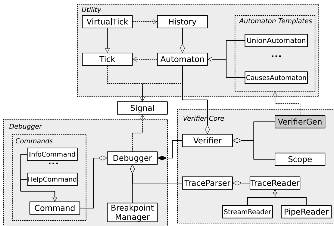
Figure 15: Verifier architecture
