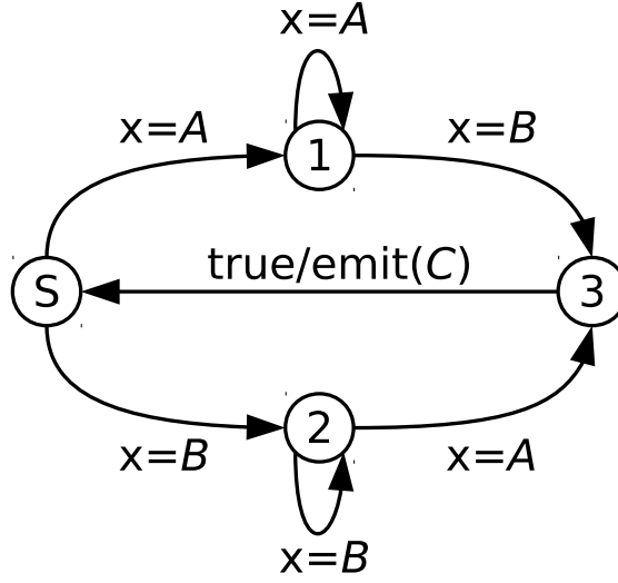
Figure 10: Clock sequence automaton
