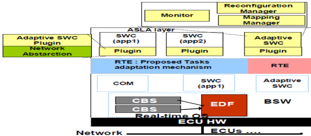
Figure 3: The ASLA architecture.
