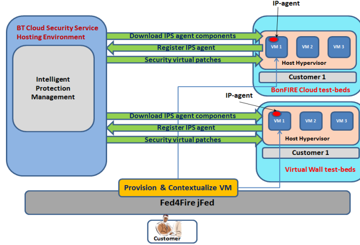
Fig. 2. Intelligent Protection provisioning architecture in Fed4FIRE
