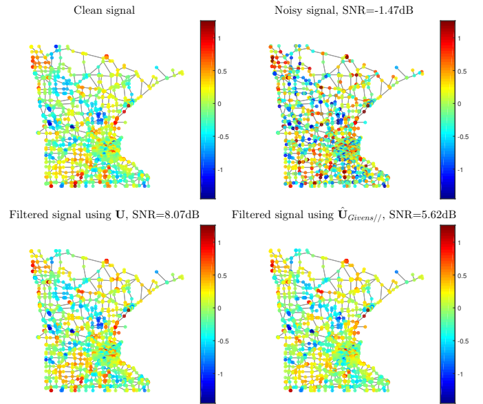
Fig. 8. Filtering example on the Minnesota road graph, the approximate FFT \hat{\mathbf{U}}_{\text{Givens}/\!/} is approximately 35 times more efficient than the true Fourier matrix \mathbf{U} .
