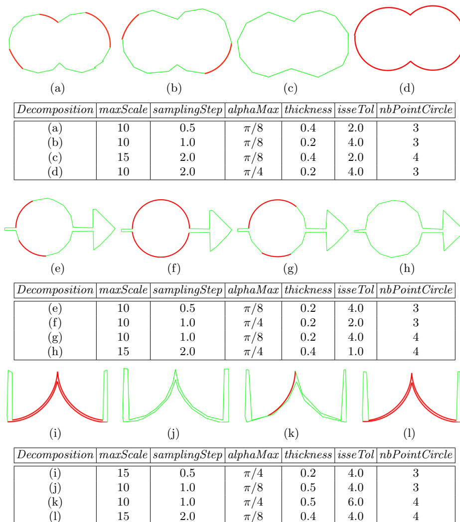
Fig. 14. Experiments on the sensibility to parameters of Fig. 10.
