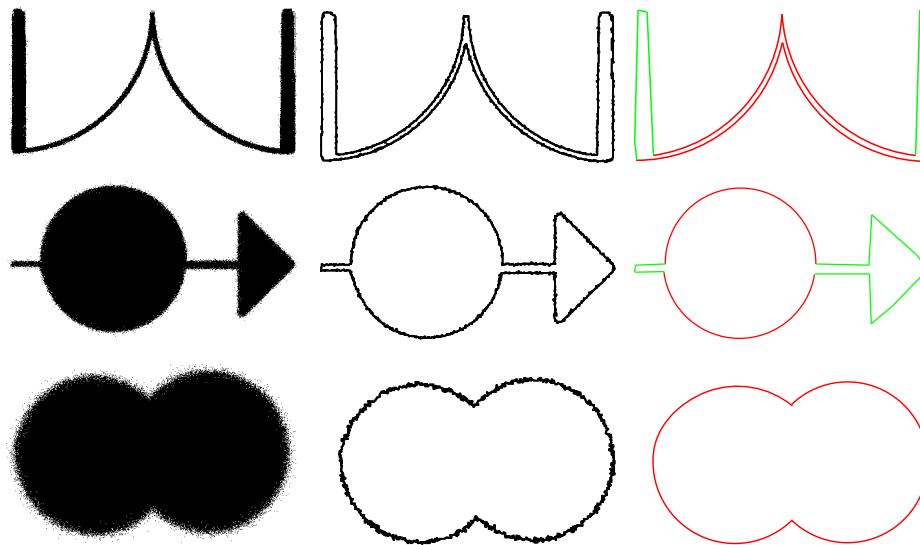
Fig. 10. Arcs and segments reconstruction of noisy curves. Left: input with Kanungo noise for \beta = 0.3 (first image), 0.5 (second image) and 0.5 (third image), middle: extracted curves, right: decomposition results.
