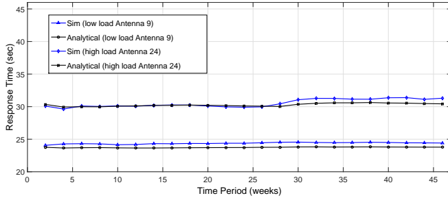
Figure 9: Analytical vs. Simulated Response Times using Arrival Rates from Real Traces.
