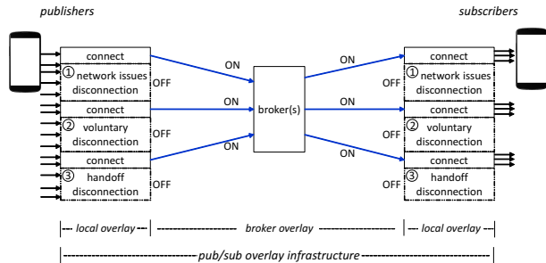
Figure 1: Peer’s connectivity behaviour.
