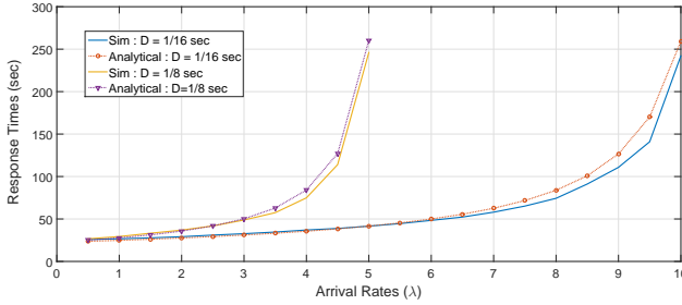
Figure 12: Response Time while traveling in metro path: Dugommier - Cité Universitaire.
