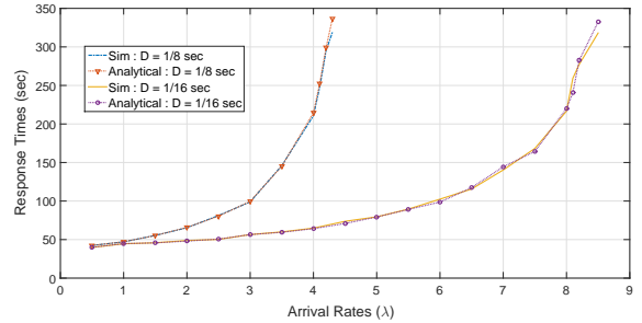
Figure 11: Response Time while traveling in metro path: Cité Universitaire - Dugommier.
