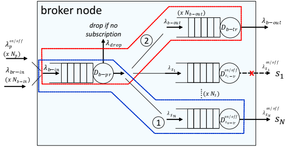
Figure 3: Pub/sub broker system model.
