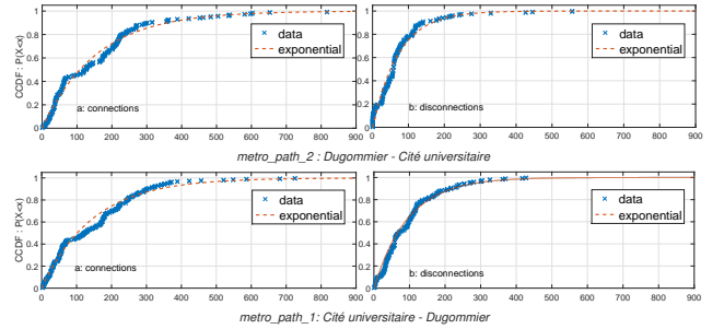
Figure 10: CCDF of connections and disconnections.
