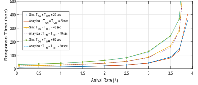
Figure 7: Analytical vs. Simulated Response Times at the ON/OFF queueing center .
