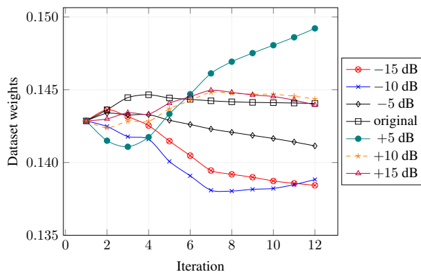
Fig. 2: Data weights learned using simulated+real development data. The sum of the weights is normalized to 1.
