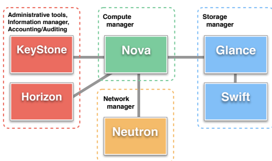
Fig. 2. OpenStack core-services
