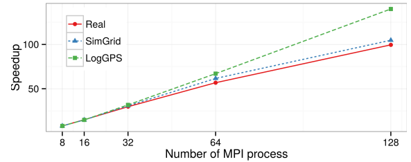
Figure 8: Prediction of the performance of BigDFT on a prototype ARM-based cluster.
