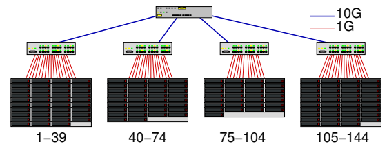
Figure 2: graphene : a hierarchical Ethernet-based cluster ( https://www.grid5000.fr/mediawiki/index.php/Nancy:Network ).
