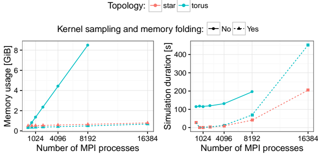
Figure 7: Simulation scalability depending on its configuration and on the workload.
