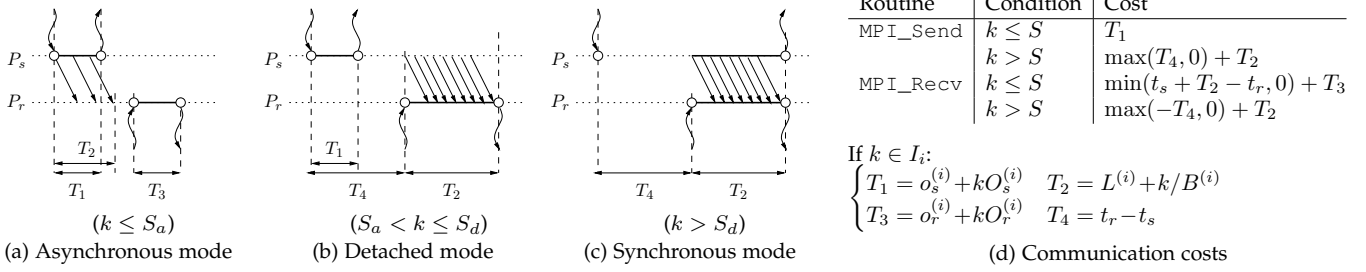
Figure 4: The "hybrid" network model of SMPI in a nutshell.
