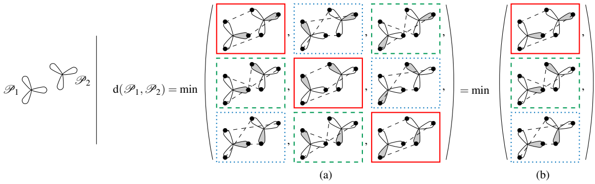
Fig. 2 Illustration of our proposed distance for a 2D object with a rotation symmetry of 2\pi/3 . (a) The distance between two poses consists in the minimum distance between two poses of an equivalent object without proper symmetry – here there are 3 possible poses of the equivalent object for each pose of the original object. The distance between poses of an object without proper symmetry corresponds to the RMS distance between corresponding object points (dashed segments). (b) Equivalently, the proposed distance can be considered as a measure of the smallest displacement from one pose to another – here there are actually only 3 different displacements between those two poses (solid, dotted and dashed boxes).
