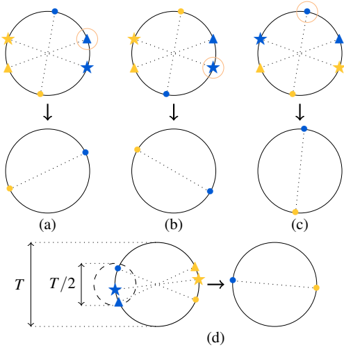
Fig. 4 Estimating the average of poses with multiple representatives: illustration with the orientation of a 2D object with a 180^\circ rotation symmetry, that can be represented by a point on a circle, or the antipodal point. We consider three poses to average (triangle, star and disk shapes). (a, b, c) The choice of a “consistent” combination of poses representatives (blue clusters) in the sense of (Gramkow 2001) is dependent of the initial choice (circled, first row), resulting potentially in different estimations of the average pose (second row). (d) We propose a definition of consistency – which is in particular satisfied when the considered representatives are close enough one an other – ensuring an unambiguous estimation of the average pose.
