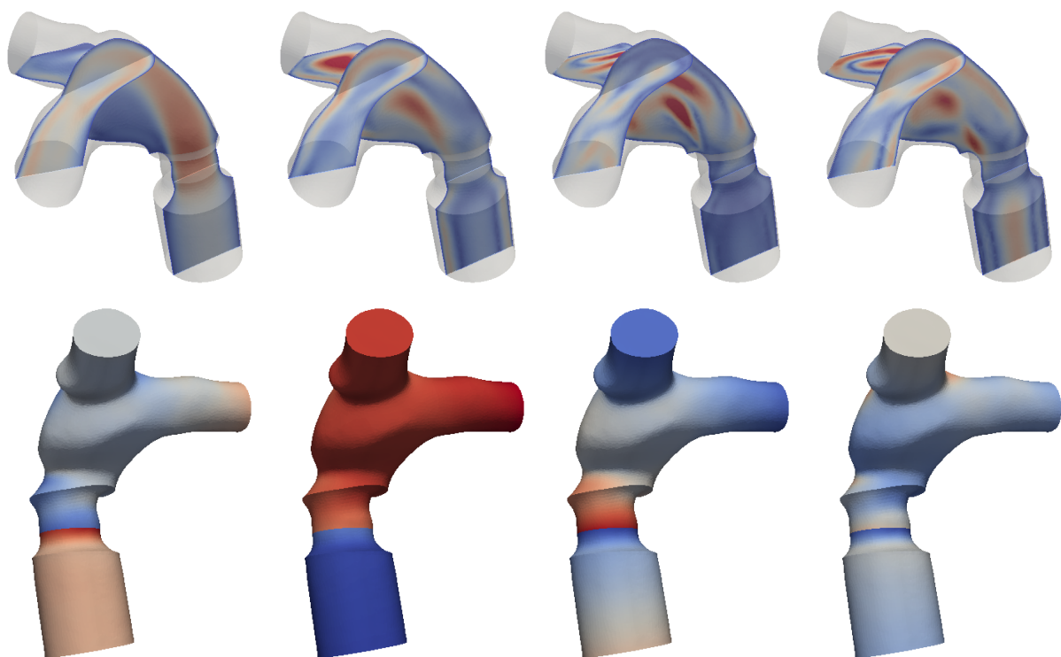
Figure 2. The four most energetic POD basis functions for velocity (in magnitude, top row) and pressure (bottom row). Notice that, by construction, POD modes are orthonormal (i.e. with unitary norm) with respect to the discrete l^2 -scalar product.
