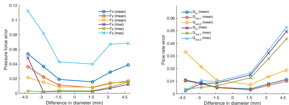
Figure 5. Average and maximum renormalized errors (1) of the reduced order model against a full finite element simulation, as a function of the diameter of the reducer. Left: Pressure forces. Right: Flow rates.
