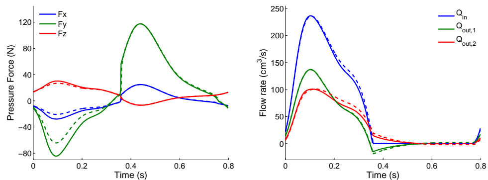
Figure 4. Continuous line: full finite element simulation; dashed line: reduced order simulation with 30 basis functions computed from the reference geometry (diameter 19 mm). Left: pressure force over time for the simulation with the smallest diameter (14 mm); Right: inlet and outlet flow rates over time for the simulation with the smallest diameter (14 mm).
