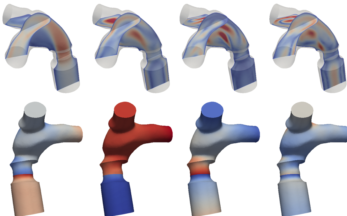
Figure 2. The four most energetic POD basis functions for velocity (in magnitude, top row) and pressure (bottom row). Notice that, by construction, POD modes are orthonormal (i.e. with unitary norm) with respect to the discrete l^2 -scalar product.
