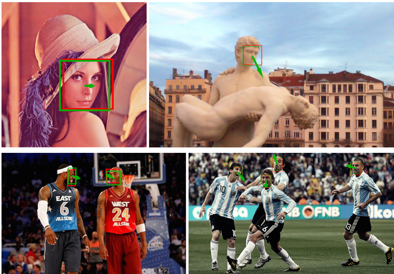
Fig. 5. Examples of simultaneous estimation of head-pose angles and of bounding-box shifts. The initial bounding box (found with an automatic face detector) is shown in red. The estimated bounding box is shown in green.
